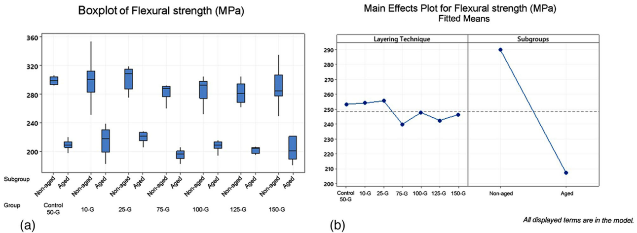
FIGURE 2 (a) Boxplot of flexural strength values obtained among the groups. (b) Main effects plot for flexural strength obtained among the groups.
