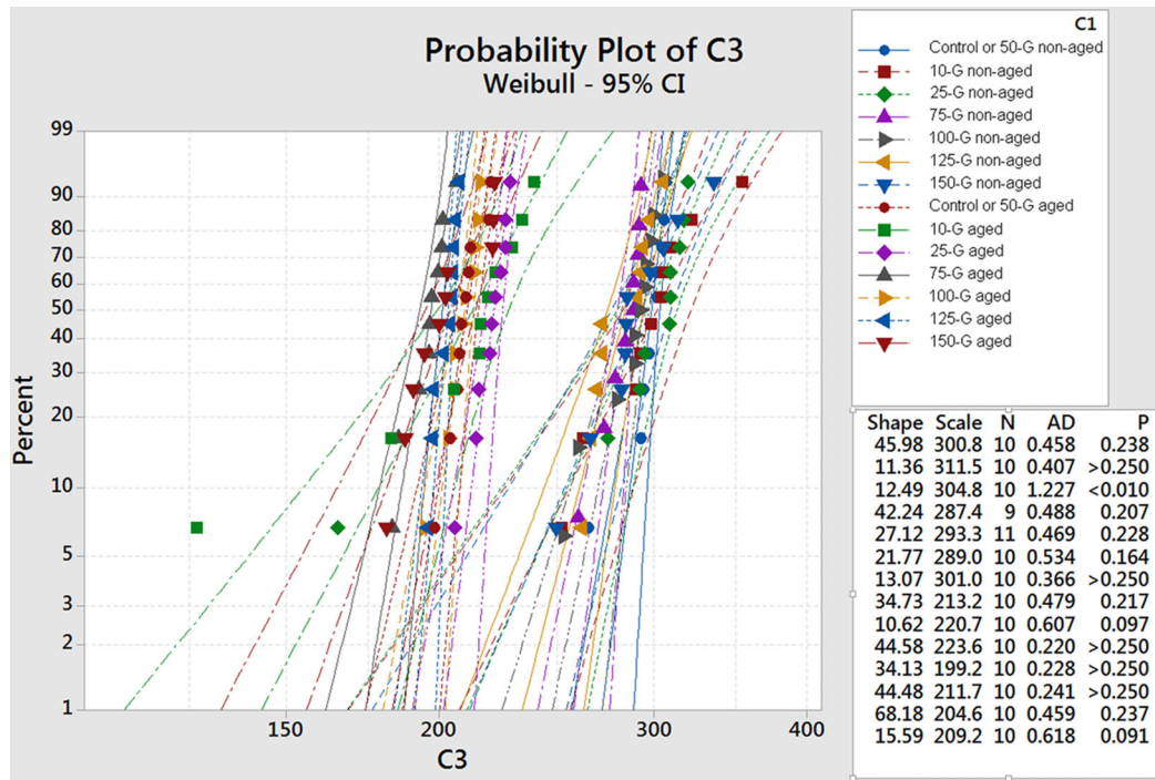
FIGURE 3 Weibull modulus for all the groups tested.
